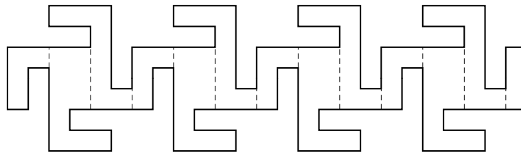
Fig. 1.3 The dashed lines show a minimum cardinality partition into at most 8-vertex pieces
