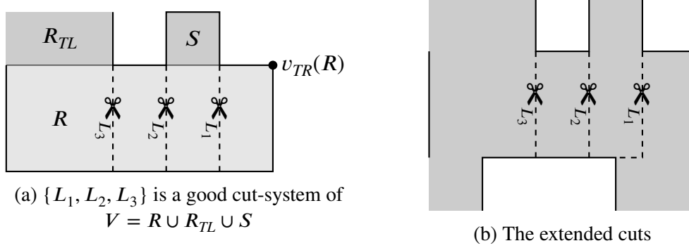
Fig. 2.8 R has one pocket
